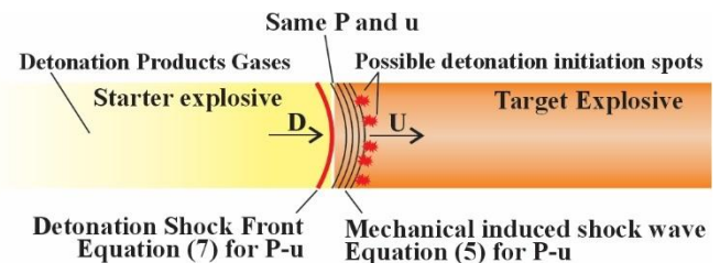
Fig. 1. Diagram of shock wave induced by a detonation shock front.
