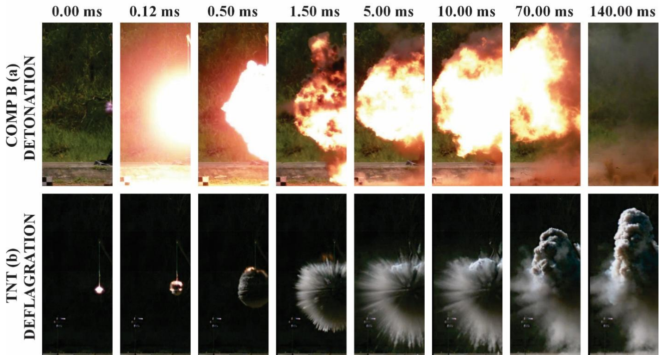
Fig. 3. High-speedy camera frames for a Comp B detonation (a) and a TNT deflagration (b). All tests presented similar results for the same explosive. The footage shows just half of the test, as the process were all symmetric. The timestamps indicate the elapsed time since initiation.
